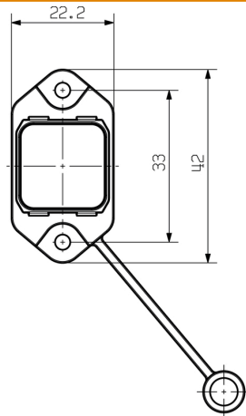
Dimensioned drawing
