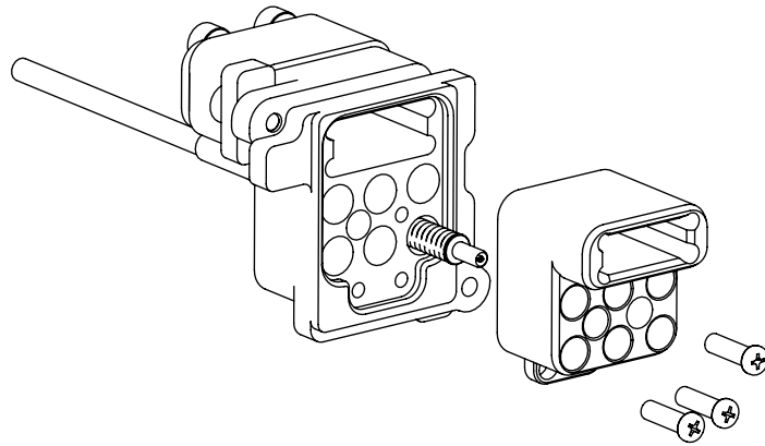
CONTACT REMOVAL - STEP 1 REMOVE FRONT PLATE AND SCREWS USING PH000 DRIVER.
