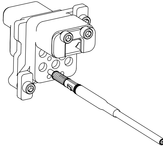
CONTACT INSERTION - STEP 1 ALIGN FEMALE (PIN) CONTACT WITH REAR RF PORT
