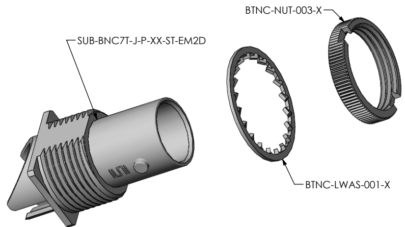
FIG 1 BNC7T-J-P-XX-ST-EM2D SHOWN
