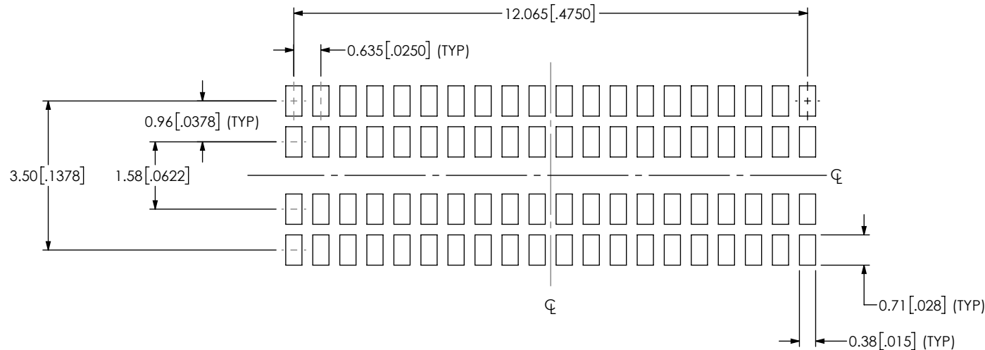
RECOMMENDED STENCIL LAYOUT STENCIL TO BE 0.127 [.0050] THICK
