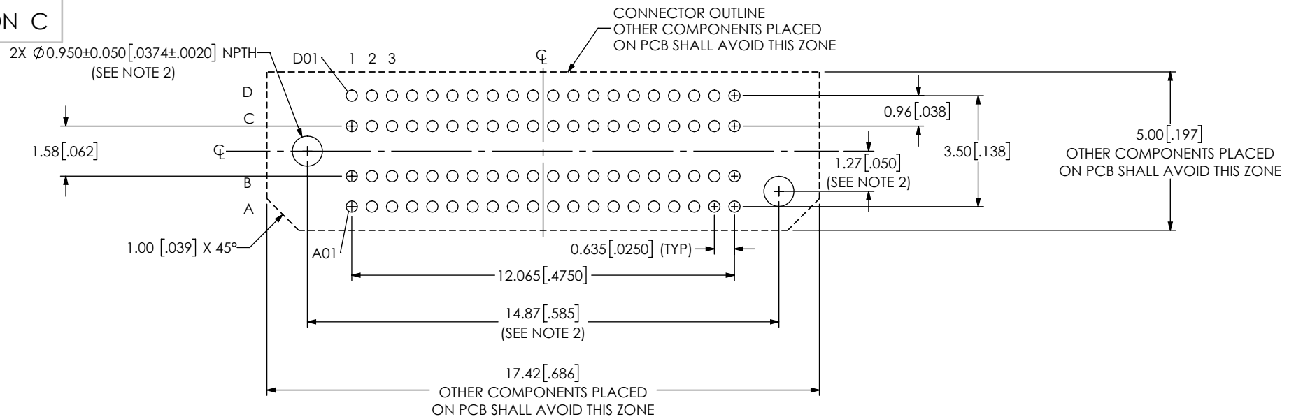
RECOMMENDED PCB LAYOUT ALL DIMENSIONS SYMMETRIC ABOUT THE CENTERLINE
