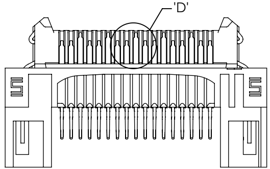
ODD ROW (DP SIDE, HOT PLUG SIDE)
