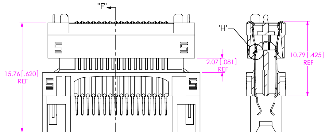
SECTION "F"- "F"
