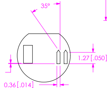
DETAIL 'M' SCALE 4 : 1
