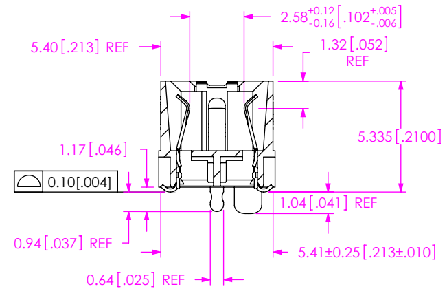
SECTION "B"- "B" SCALE 4 : 1
