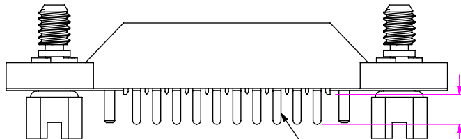
FIG 9 -01-DS: DUAL SCREW DOWN WITH -01 LEAD STYLE (SAME AS FIG 8, DIFFERENT AS SHOWN)
