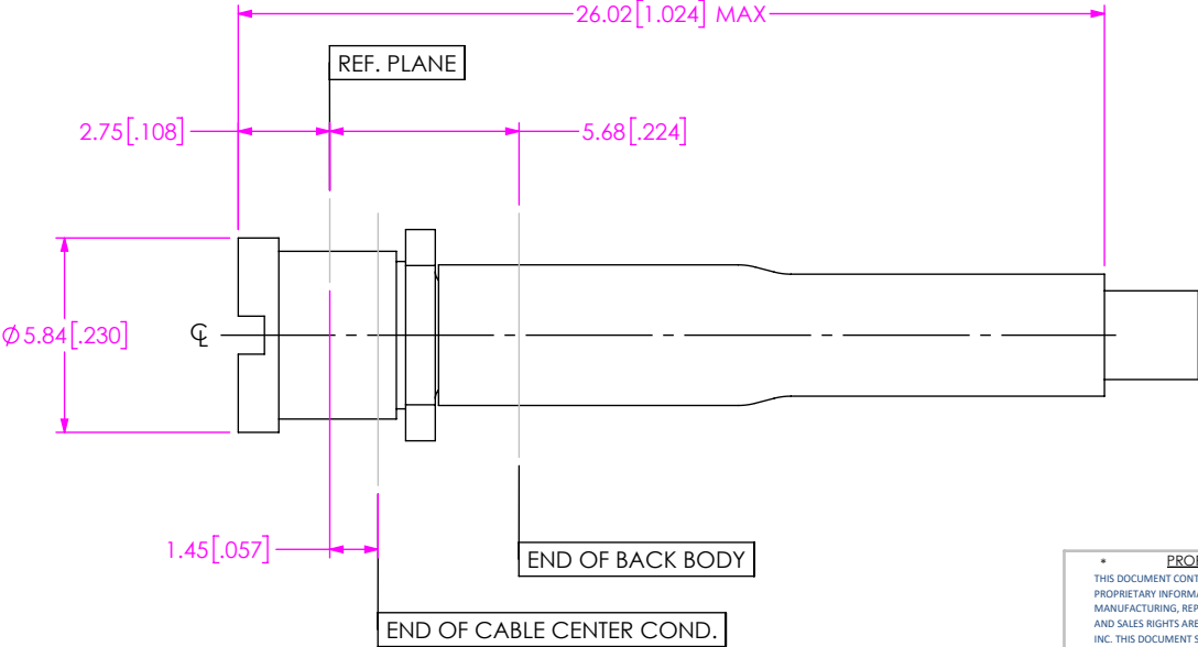
FIG 14 -00BC, -00BF, -00BL, -00BS SHOWN (PROTECTIVE CAP NOT SHOWN FOR CLARITY)
