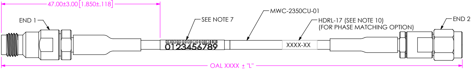
FIG 1 RF23C-24SJ-92SP-XXXX-X-XX SHOWN (PROTECTIVE CAPS NOT SHOWN FOR CLARITY)
