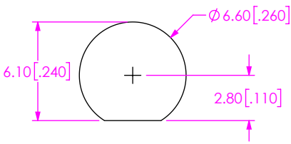
RECOMMENDED PANEL LAYOUT 3.80 [.150] MAX. PANEL THICKNESS
