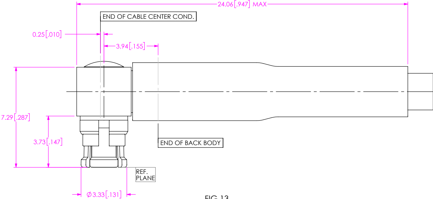
FIG 13 -00MJ SHOWN (PROTECTIVE CAP NOT SHOWN FOR CLARITY)
