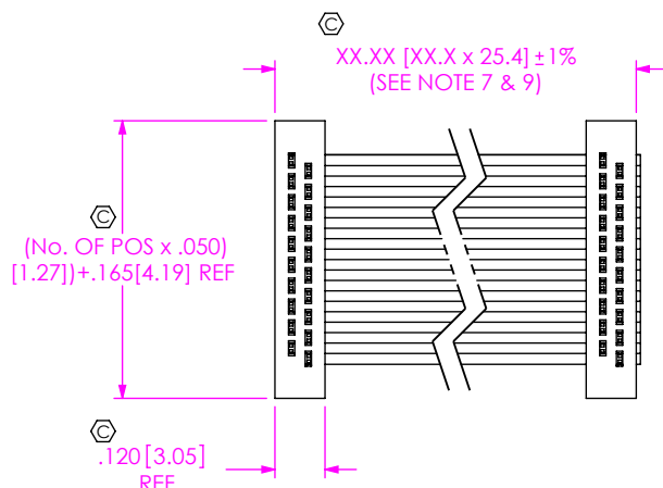
FIG 1 (FFMD-10-D-XX.XX-01-X SHOWN)
