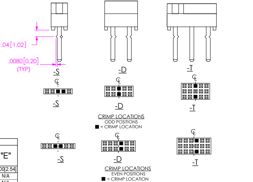
FIG 2 -LL: LOCKING LEAD OPTION LOCATED ON OR ABOUT CENTERLINE [N/A IN 1 OR 2 POSITION SINGLE ROW] F:\DWG\SW\Exisprod\Assembly\100\ESQ-1XX-XX-X-XXX-XX-X-XX.slddrw
