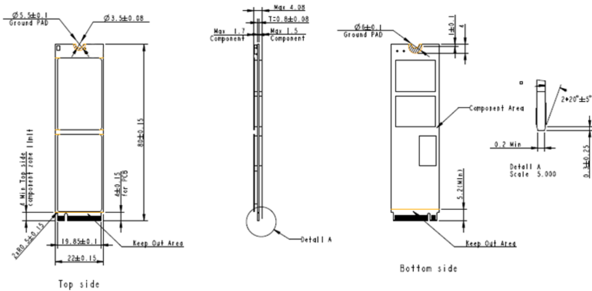
Figure 9-1 Physical Dimensions
