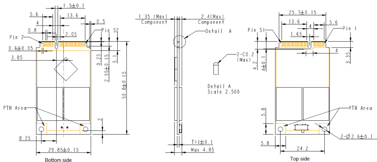
Figure 9-1 Physical Dimensions
