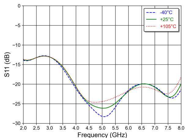
TX Return Loss in TX ON state
