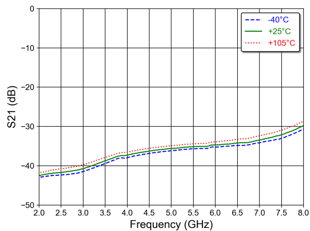
ANT to RX Isolation 13
