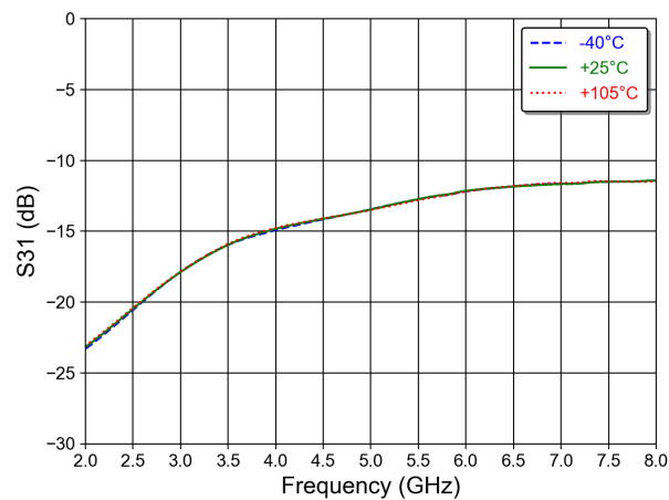
ANT to TX Isolation
