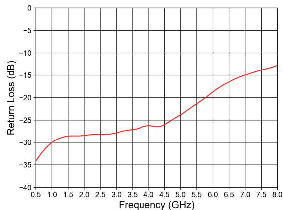
RX Return Loss in RX ON state
