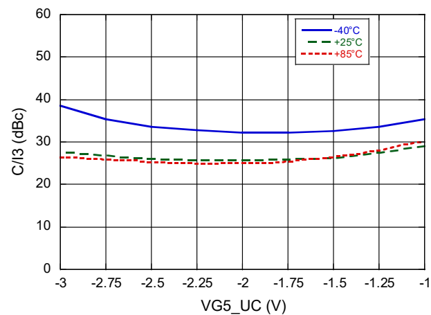
C/I3 vs. Mixer Bias, RF = 86 GHz
