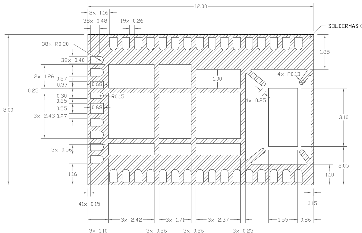
Bottom Layer Viewed From The Top
