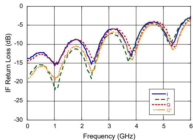
All IF Return Loss at +25°C
