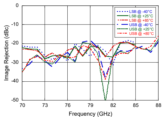
Image Rejection at IF = 2.25 GHz
