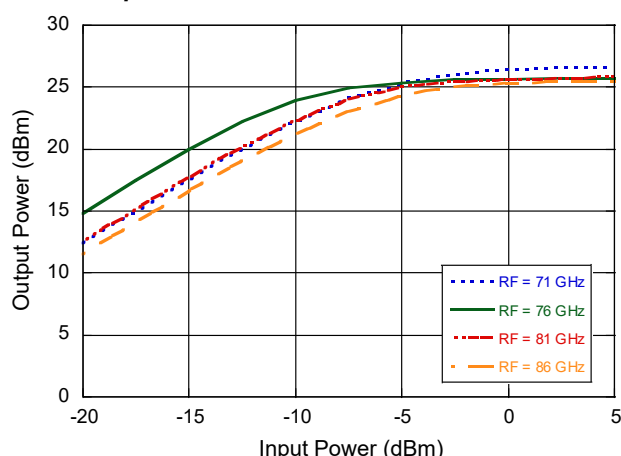
Pout vs. Input Power at +85°C
