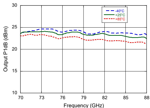
P1dB at Nominal Bias, IF = 700 MHz
