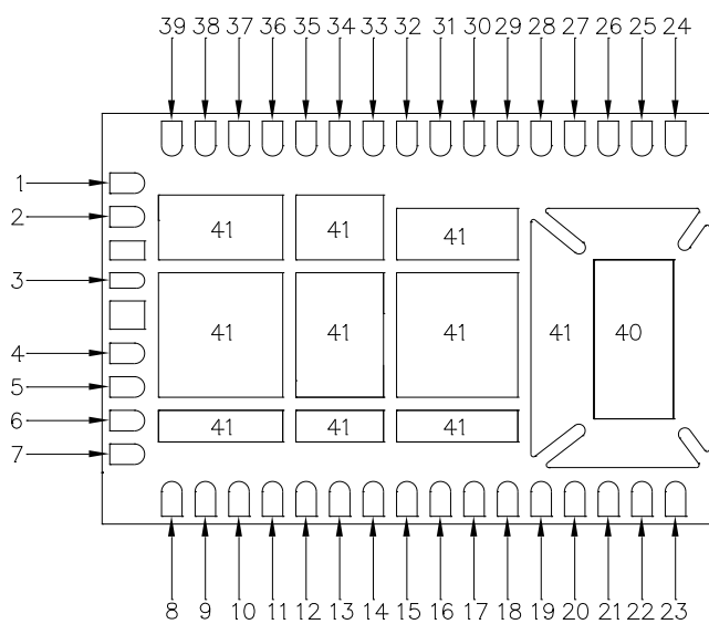
Bottom Layer Viewed From The Top
