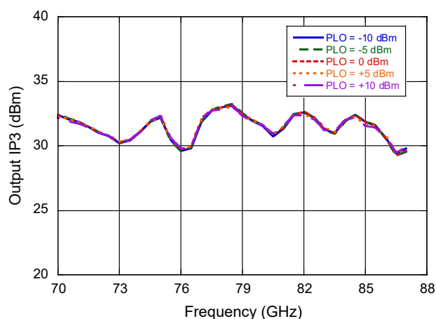
OIP3 vs. LO Power at IF = 21.4 and 26.0 MHz, +25°C
