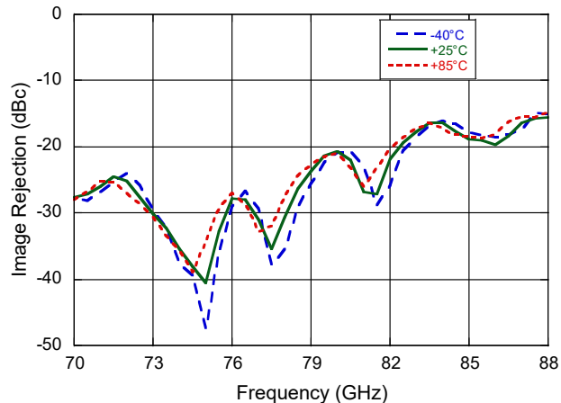
Image Rejection at IF = 700 MHz
