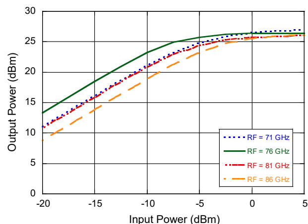
Pout vs. Input Power at +25°C
