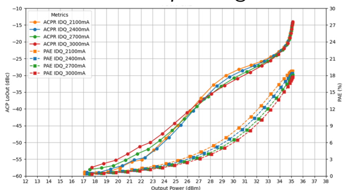
ACP LoOut and PAE vs. Output Power @ 30.0 GHz
