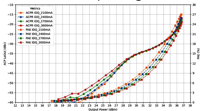
ACP LoOut and PAE vs. Output Power @ 27.5 GHz
