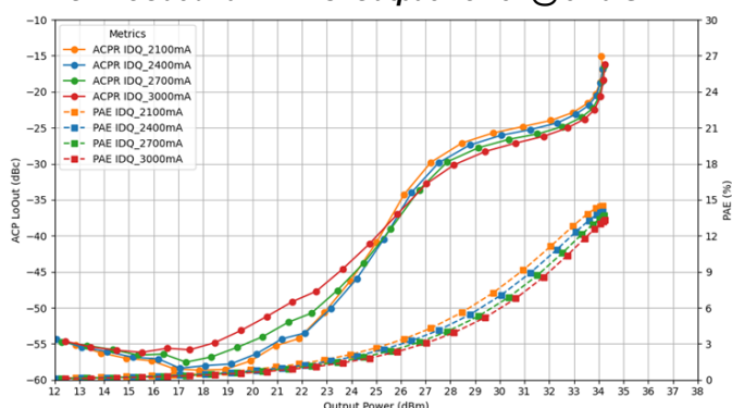
ACP LoOut and PAE vs. Output Power @ 31.0 GHz
