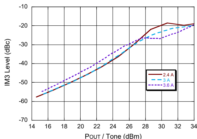
IM3 vs. Output Power @ 30 GHz, @ I_{dsq}=2.4 A, 3A and 3.6A
