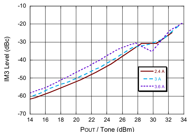
IM3 vs. Output Power @ 29 GHz, @ I_{dsq}=2.4 A, 3A and 3.6A
