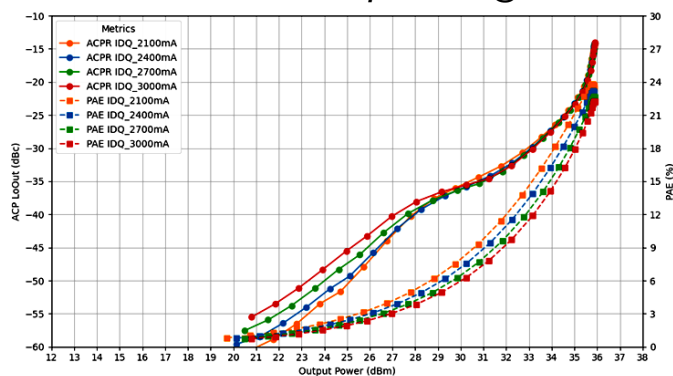
ACP LoOut and PAE vs. Output Power @ 29.0 GHz
