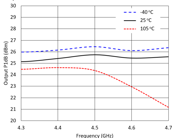
Output P_{1dB}^{11} , 4.3 - 4.7 GHz
