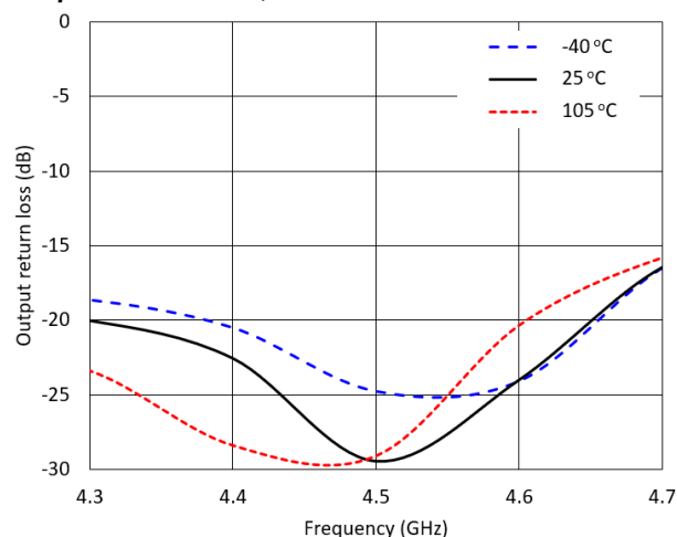
Output Return Loss, 4.3 - 4.7 GHz
