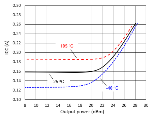
ICC vs. Output power 11 , 4.2 GHz
