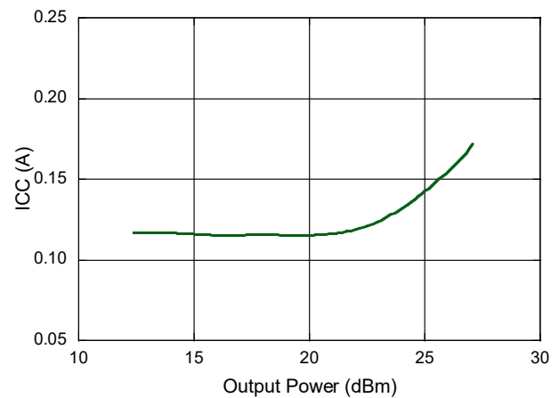
ICC vs. Output Power: 3.5 GHz, +25°C
