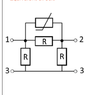
Equivalent circuit
