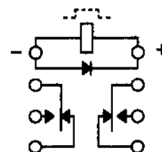
TERMINAL VIEW
