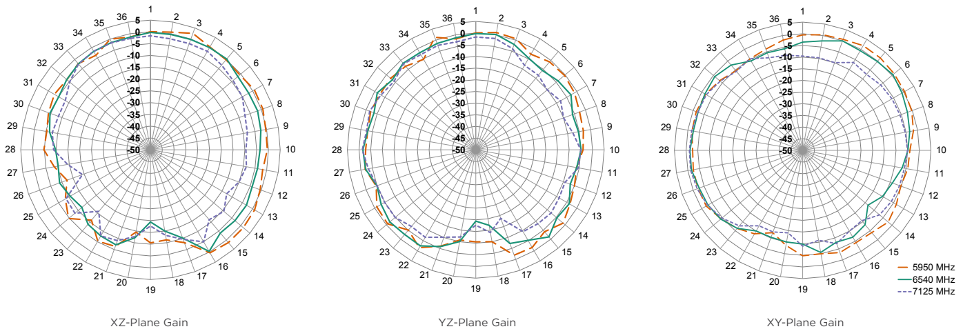
Figure 8. ANT-W63-MSA-TH1 Antenna Radiation Patterns
