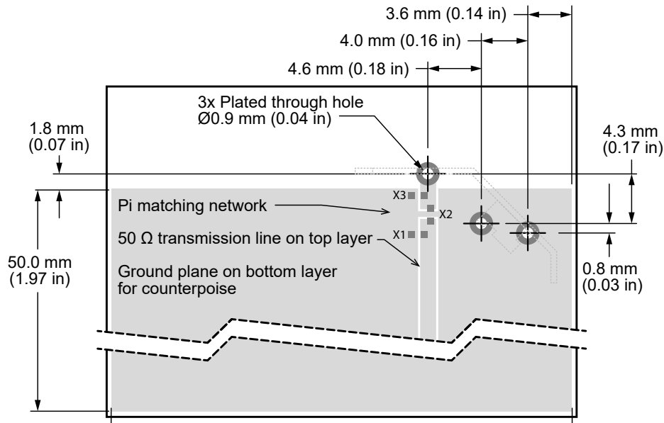
Figure 9. Matching Network Recommendation
