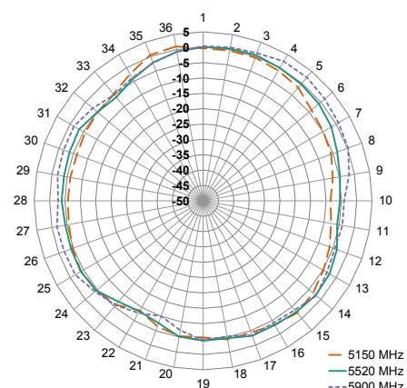
XY-Plane Gain
