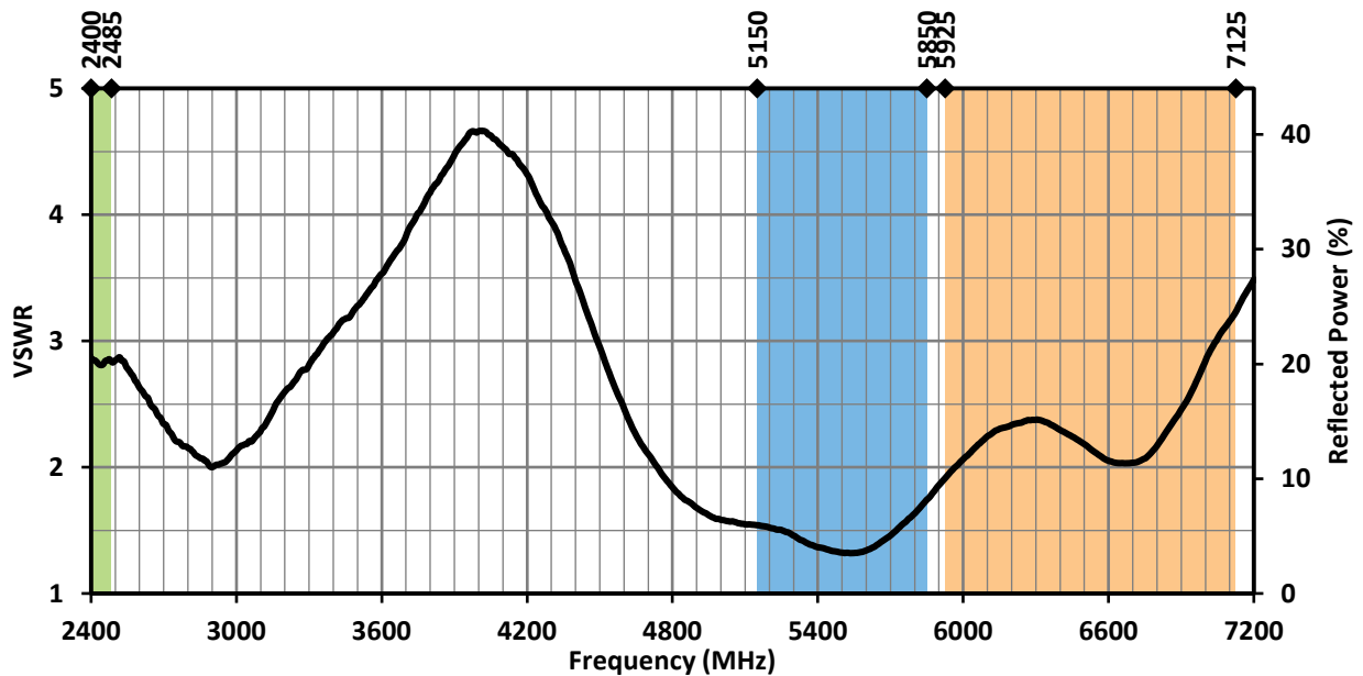
Figure 3. ANT-W63-MSA-TH1 Antenna VSWR with Frequency Band Highlights
