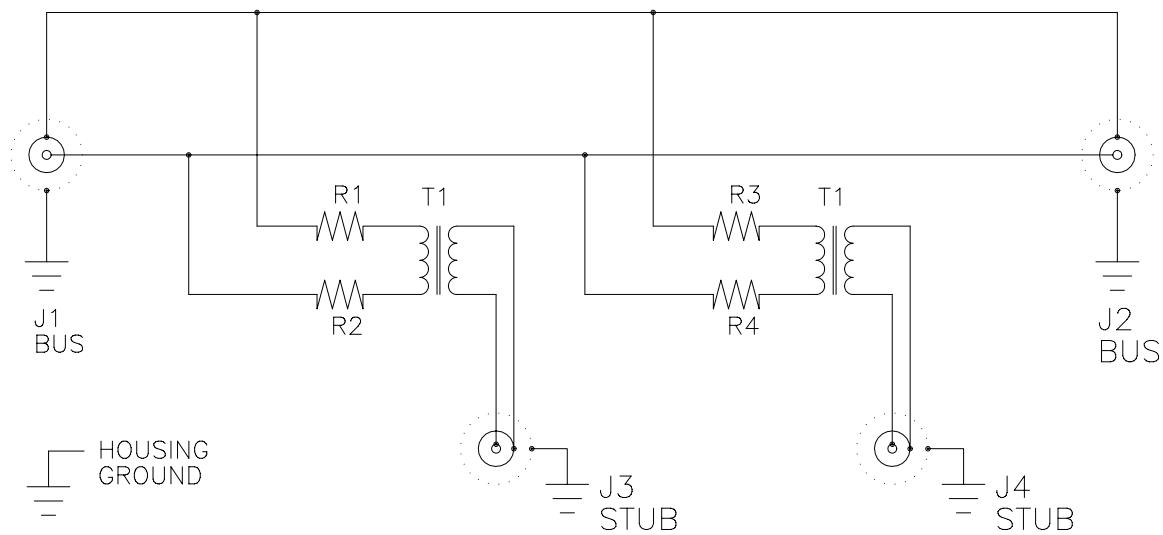
SCHEMATIC DIAGRAM
