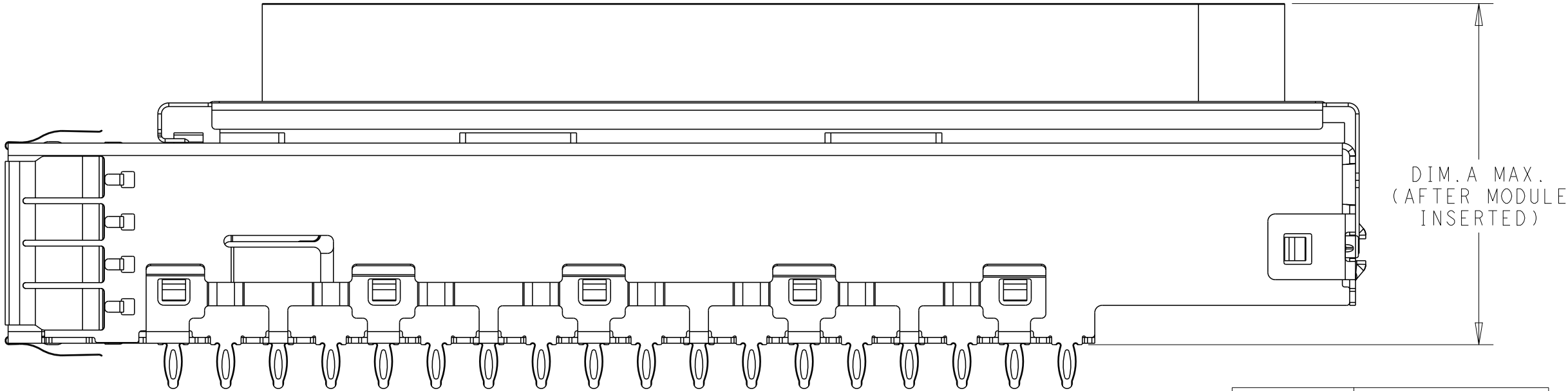
2293277-2&2293277-7/1-2293277-0 OTHER DIMENSIONS SAME AS 2293277-1 SCALE 3:1
