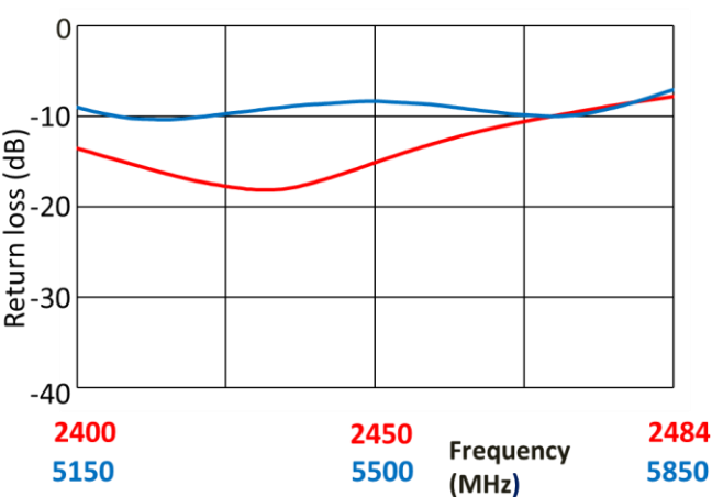
Return Loss
