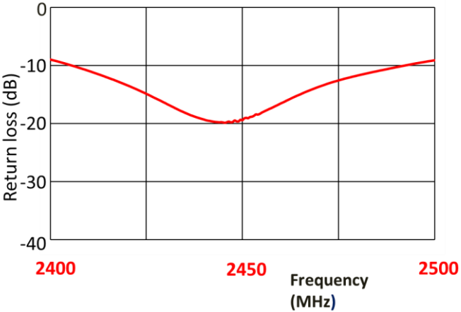
Return Loss
