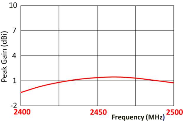
Peak Gain
