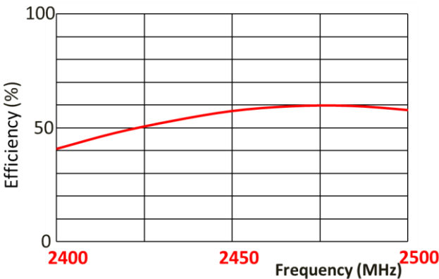
Efficiency
