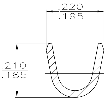
SECTION C-C
