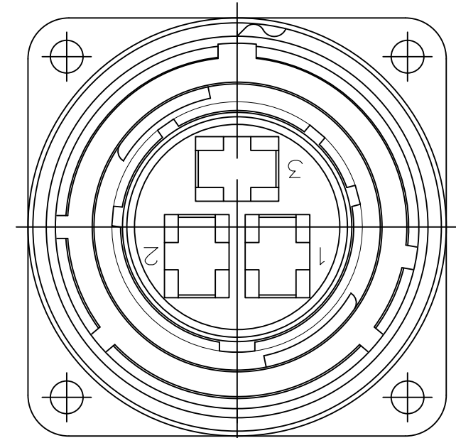
DETAIL F
