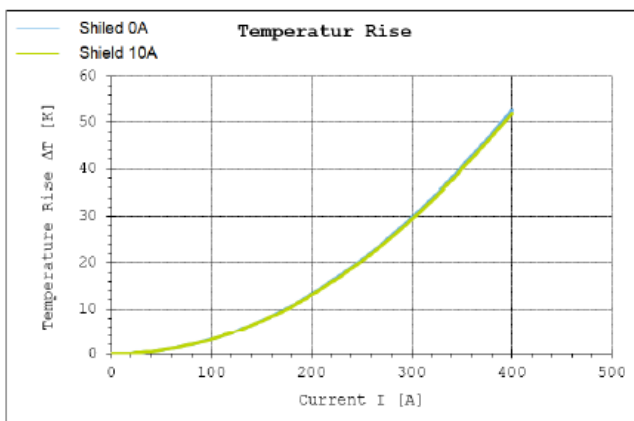
95mm 2 3pos Derating and temperature rise – derating with housing
