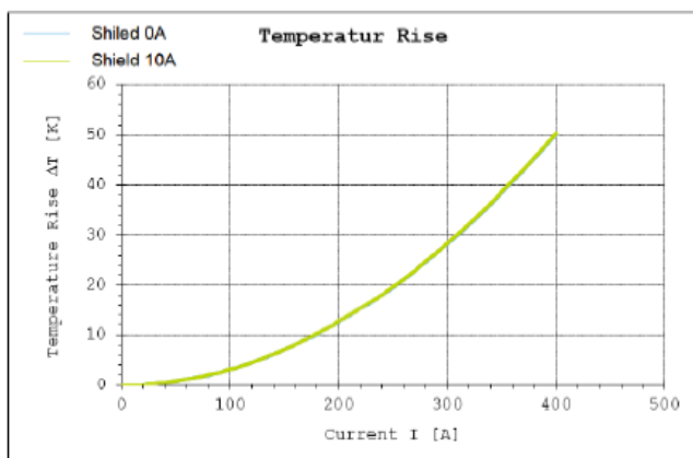
95mm 2 2pos Derating and temperature rise – derating with housing
