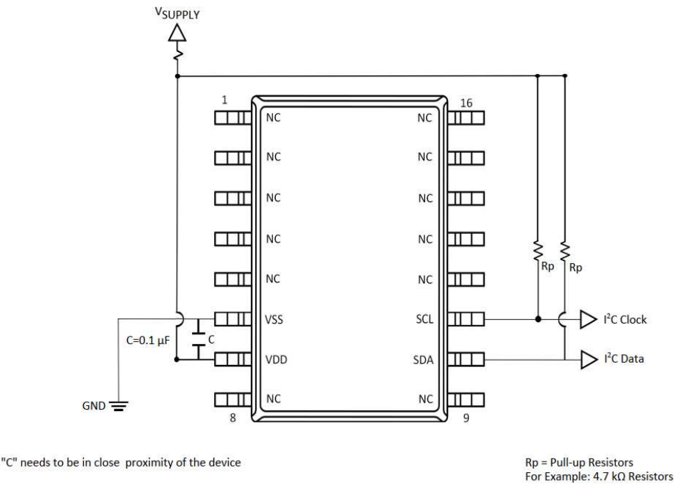
SM9541 + Family Applications Circuit
