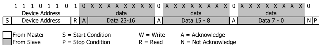
Figure 9: I 2 C answer from MS5837.
