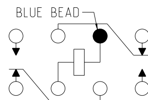
TERMINAL VIEW
