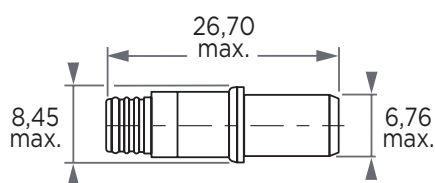
Male contact
