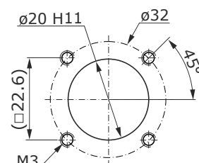
Mounting Hole
