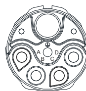
Contact Arrangement socket, code 13 mating view
