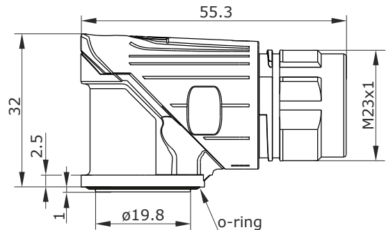
Main Dimensions receptacle angled
