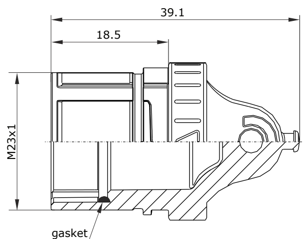
Main Dimensions sealing plug
