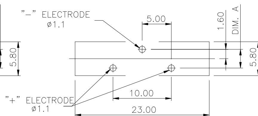
△6. RECOMMENDED PCB HOLE LAYOUT PCB TOLERANCE ±0.05
