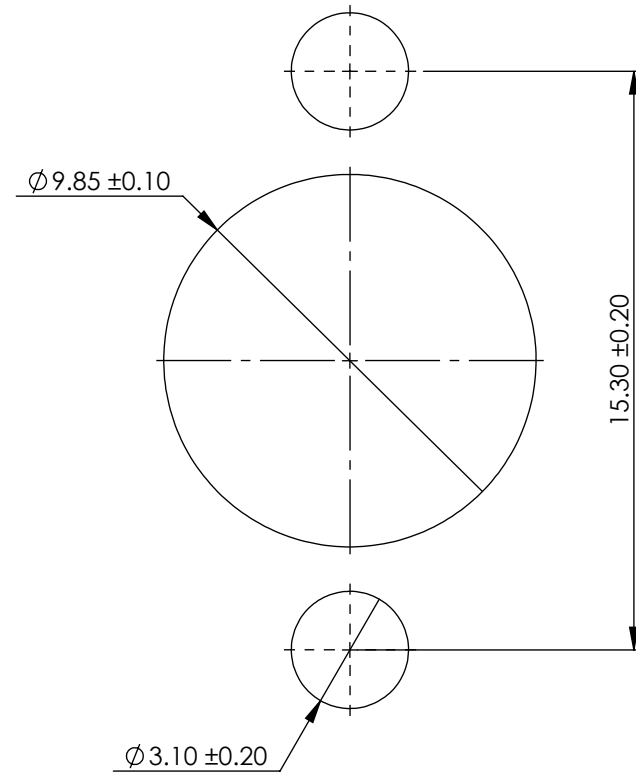
RECOMMENDED PANEL CUT OUT DETAIL
