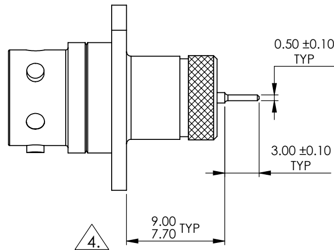
VIEW SHOWING CONNECTOR FITTED WITH PCB TAIL CONTACTS
