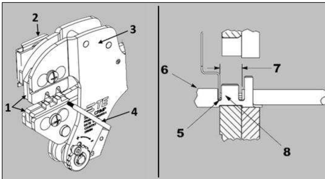
Figure 2: Crimping
