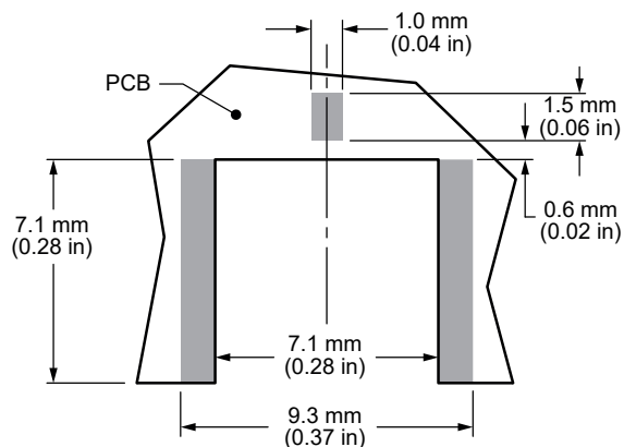
Figure 2. Recommended PCB Footprint for the CONSMA024-G Connector
