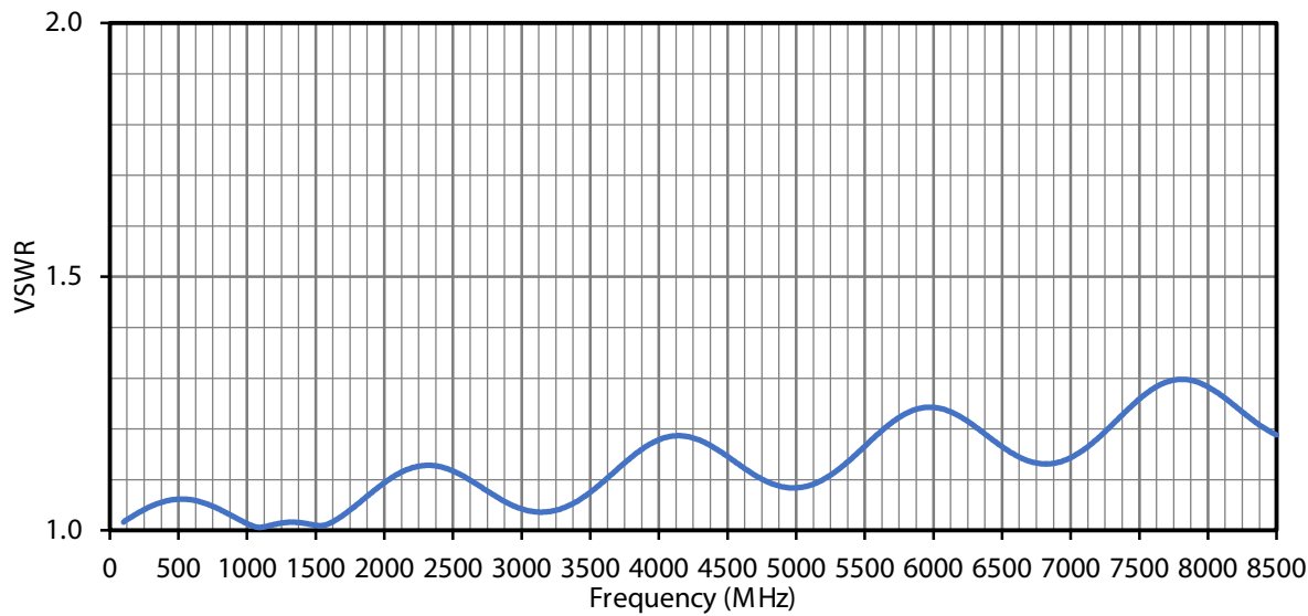
Figure 4. VSWR for the CONMMCX013 Connector
