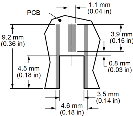
Figure 2. Recommended PCB Footprint for the CONMMCX013 Connector
