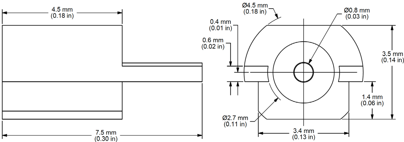
Figure 1. Product Dimensions for the CONMMCX013 Connector
