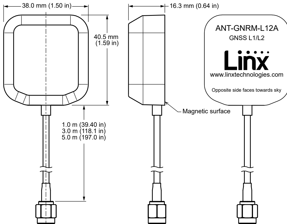
Figure 1. ANT-GNRM-L12A Series Antenna Dimensions
