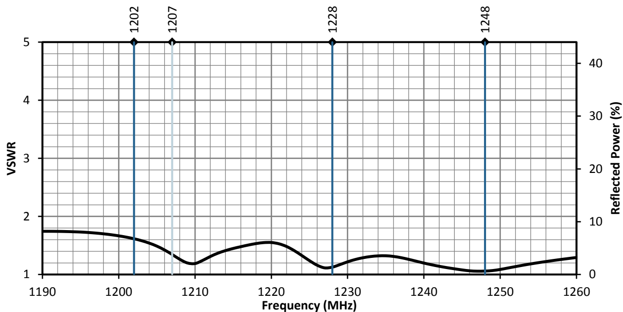
Figure 4. ANT-GNRM-L12A Series Antenna VSWR, L2 Band
