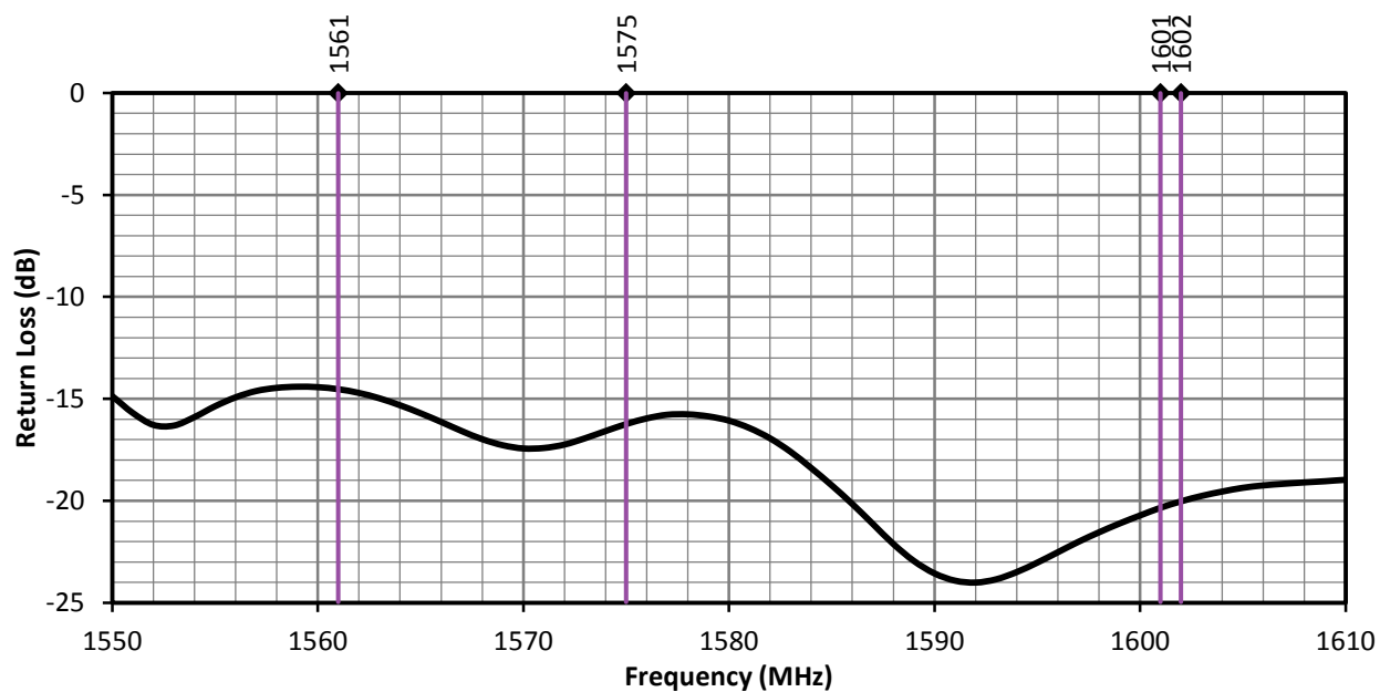
Figure 5. ANT-GNRM-L12A Series Antenna Return Loss, L1 Band
