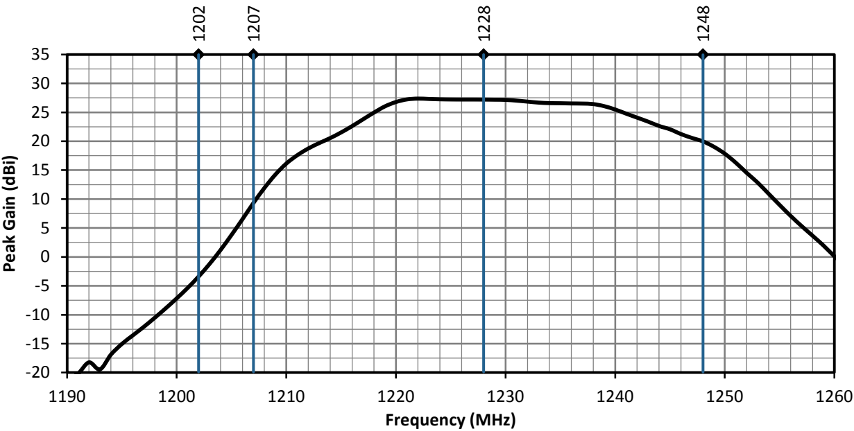
Figure 8. ANT-GNRM-L12A Series Antenna Peak Gain, L2 Band
