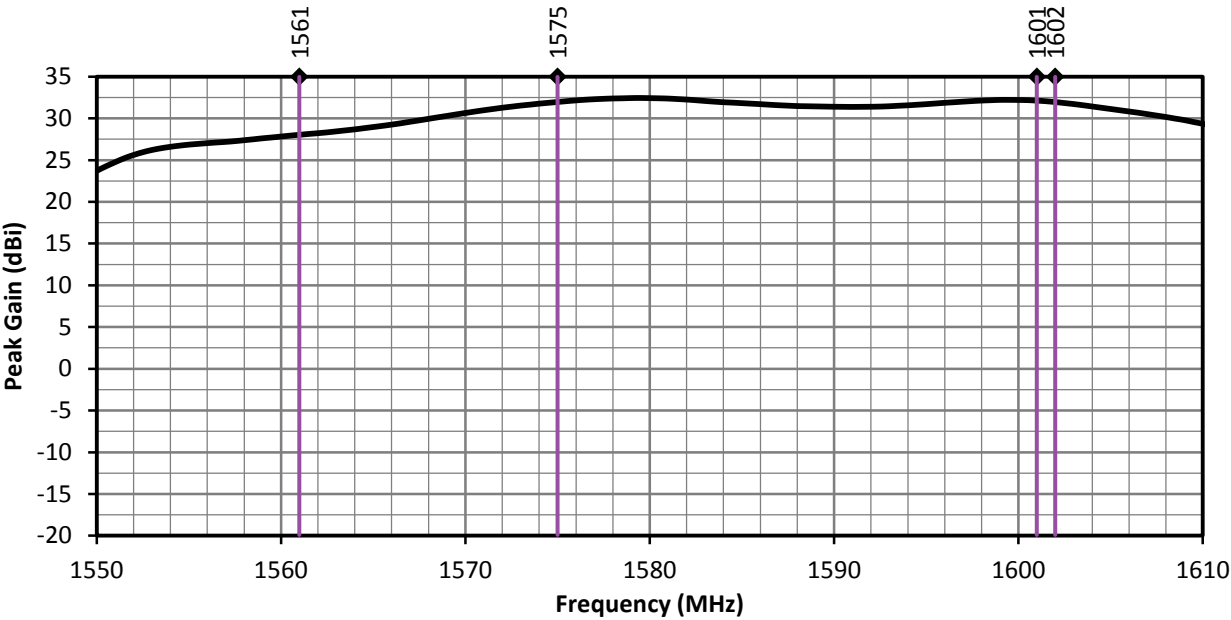
Figure 7. ANT-GNRM-L12A Series Antenna Peak Gain, L1 Band
