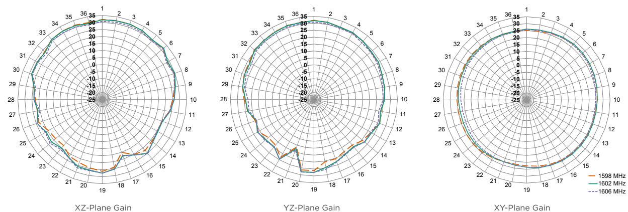
Figure 11. ANT-GNRM-L12A Radiation Patterns
