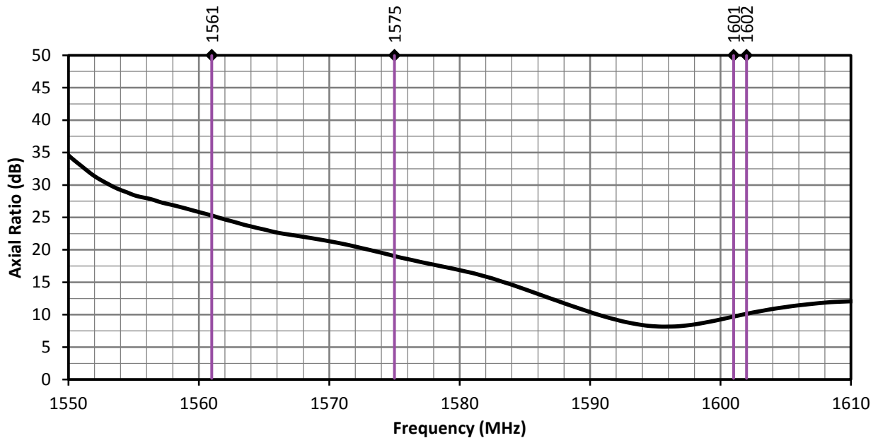
Figure 9. ANT-GNRM-L12A Series Antenna Axial Ratio, L1 Band
