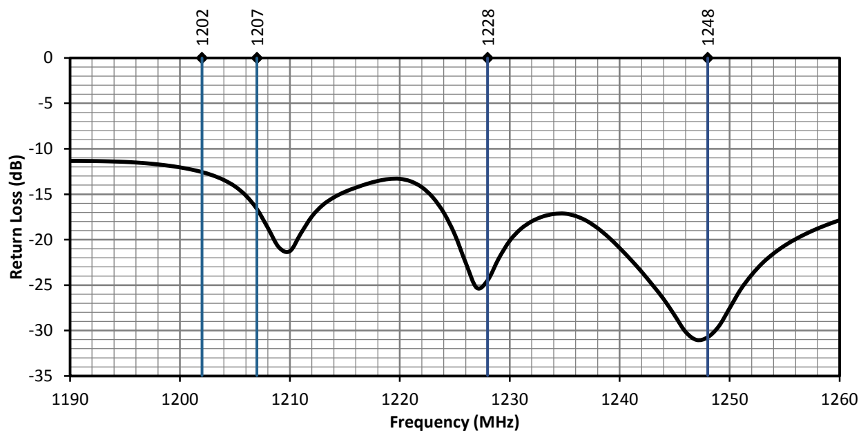
Figure 6. ANT-GNRM-L12A Series Antenna Return Loss, L2 Band
