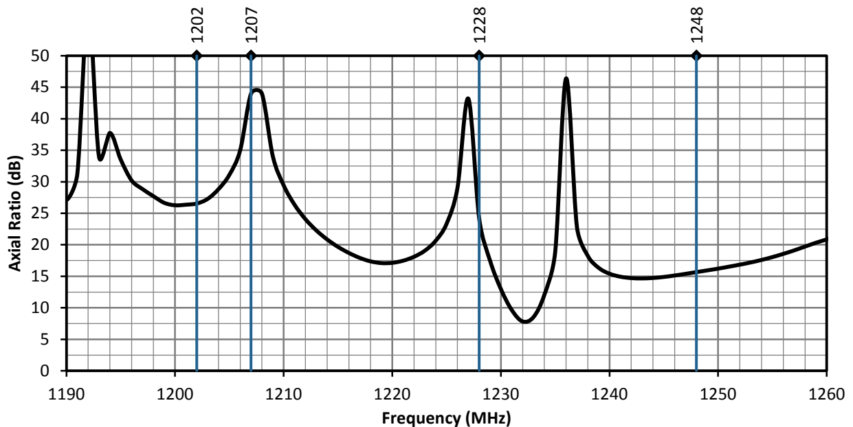
Figure 10. ANT-GNRM-L12A Series Antenna Axial Ratio, L2 Band
