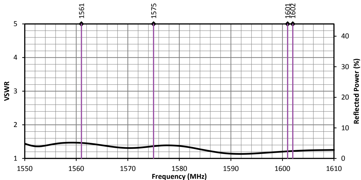
Figure 3. ANT-GNRM-L12A Series Antenna VSWR, L1 Band
