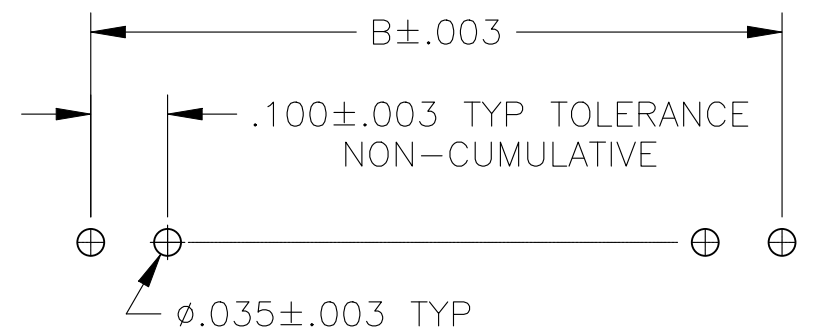
RECOMMENDED HOLE LAYOUT
