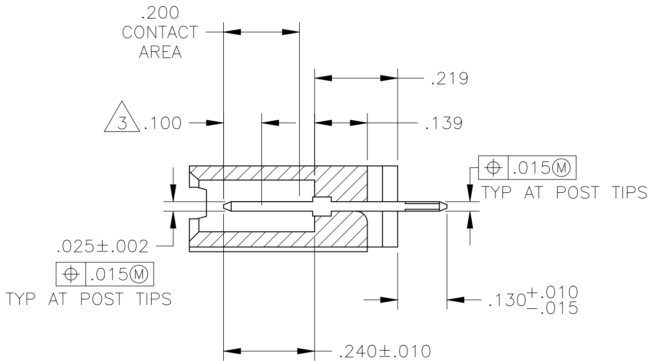
SECTION X-X
