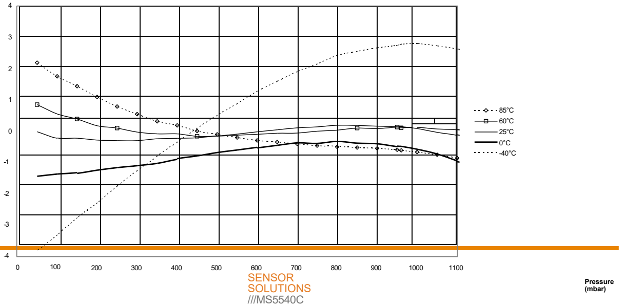
Absolute Pressure Accuracy after Calibration, 2nd order compensation
