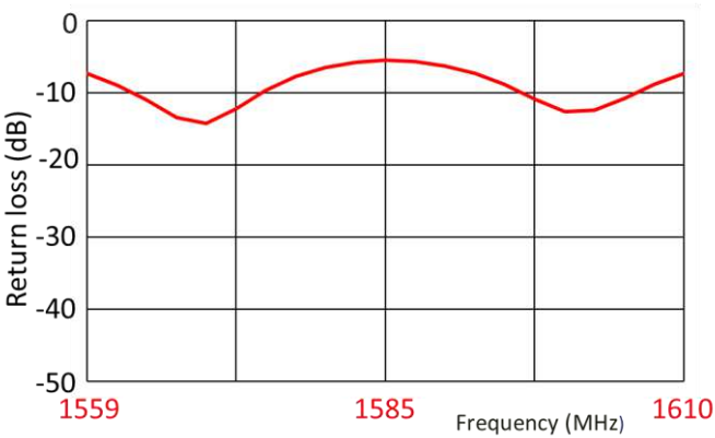
Return Loss
