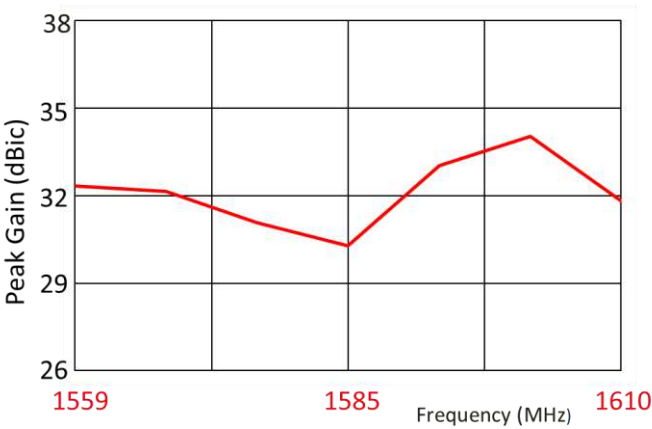
Peak Gain
