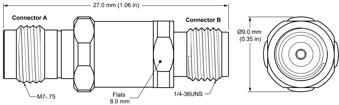
Figure 1: Product Dimensions for the ADP-2.4F-2.92F Adapter
