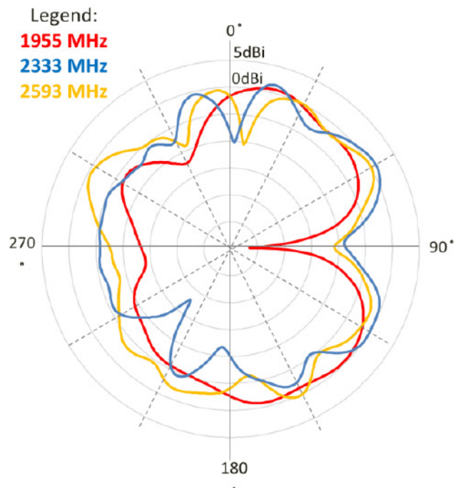
Elevation 2(YZ)
