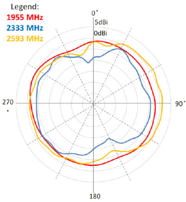
Elevation 1(XZ)
