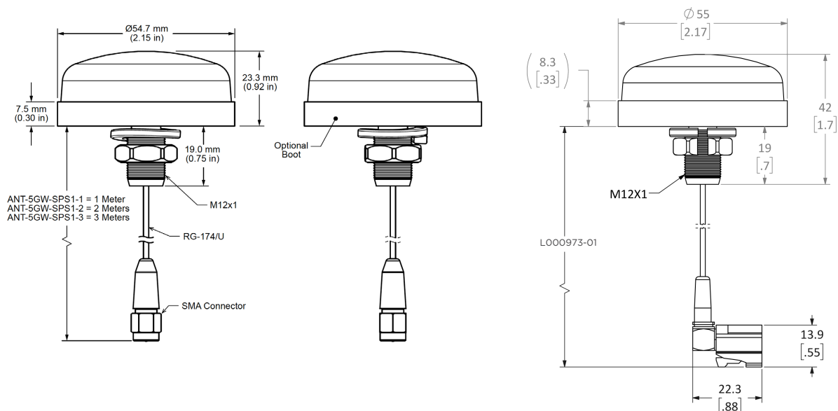
Figure 1. ANT-5GW-SPS1 Series Dimensions
