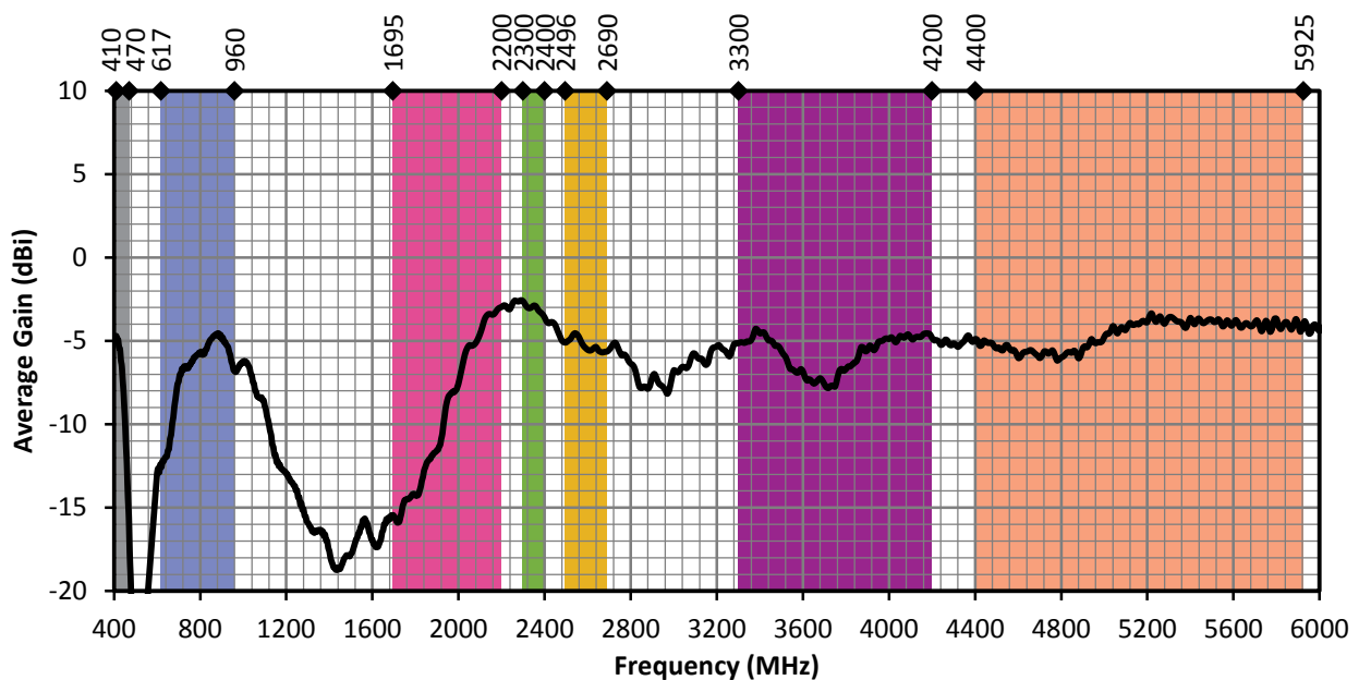
Figure 5. ANT-5GW-SPS1 Antenna Average GainStraight
