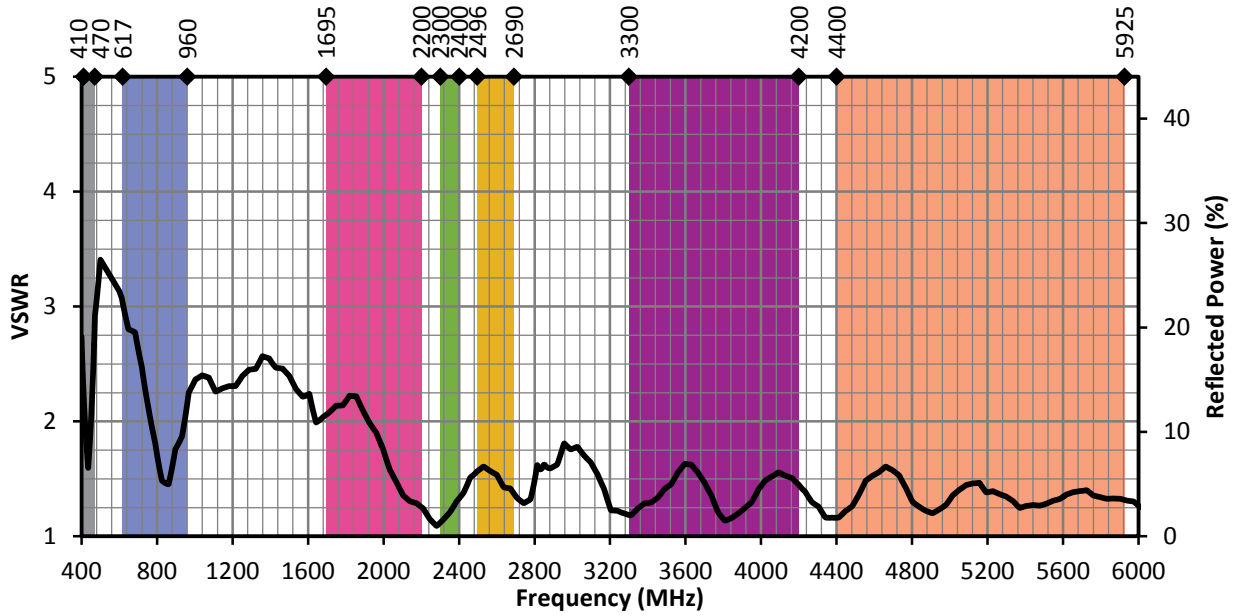
Figure 2. ANT-5GW-SPS1 VSWR
