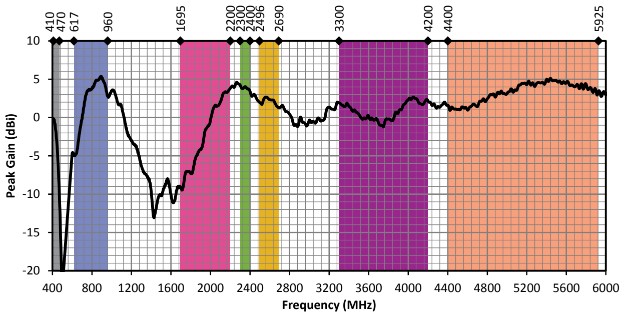
Figure 4. ANT-5GW-SPS1 Peak Gain
