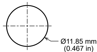
Figure 8. ANT-5GW-SPS1 Mounting Hole Dimensions Patterns
