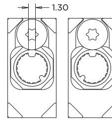
2828454-4 (Mates with x-2828999-4) 2828454-6 (Mates with x-2828999-6)
