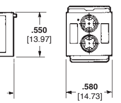
Cap Rear
