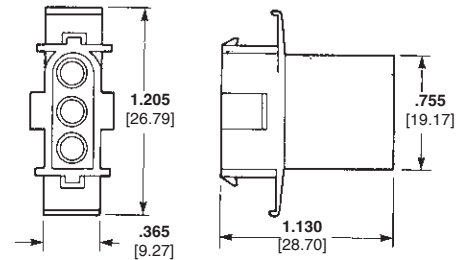
Pin Housing (Cap)
