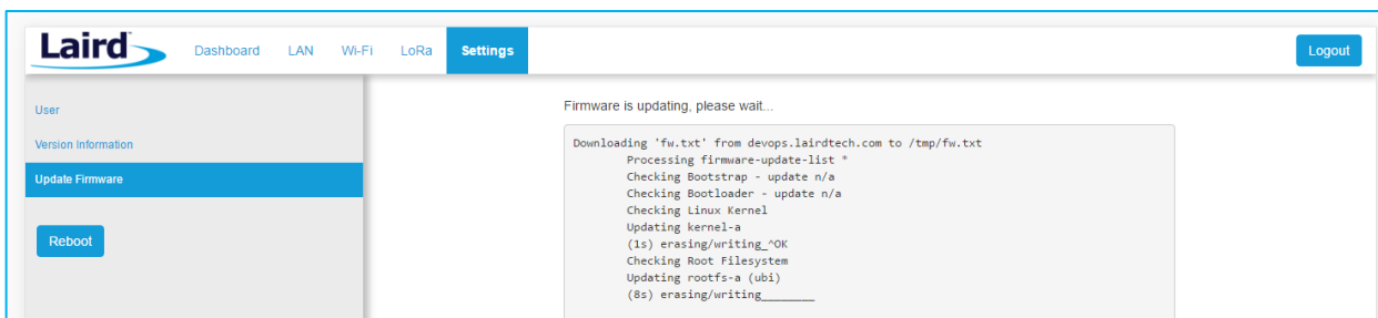
Figure 36: Progress indicator
