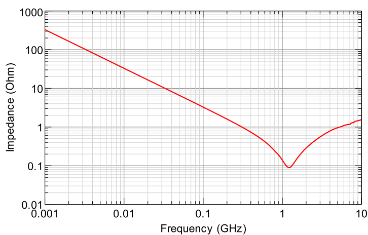
Figure 2 - 470pF WLSC measurement results (Impedance characteristic versus Frequency in shunt mode)
